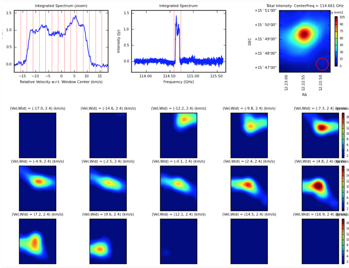
Figure 58: An example of a channel map.
