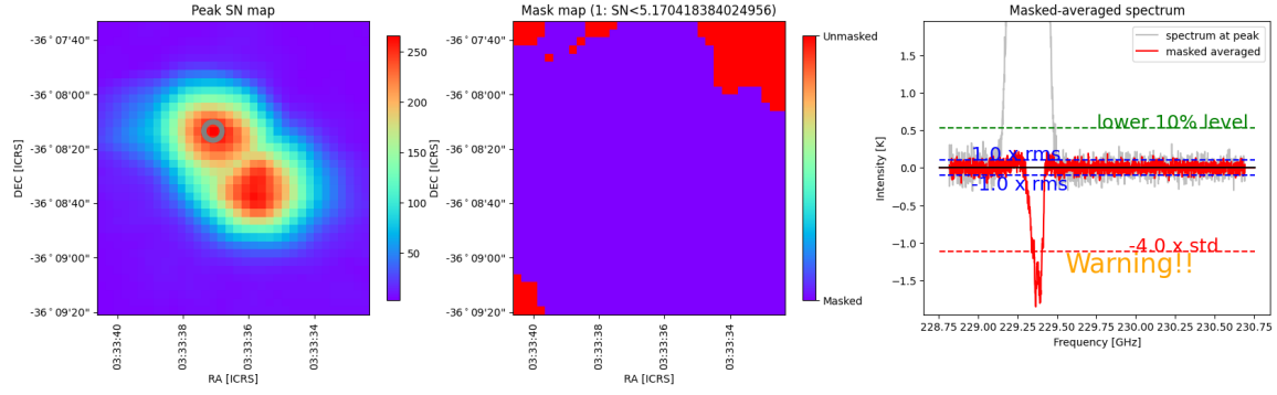
Figure 2: An example of the contamination plot for the case the OFF position is contaminated by the astronomical signal. The spectrum with the negative peak indicates that the OFF position is contaminated by the astronomical signal.
