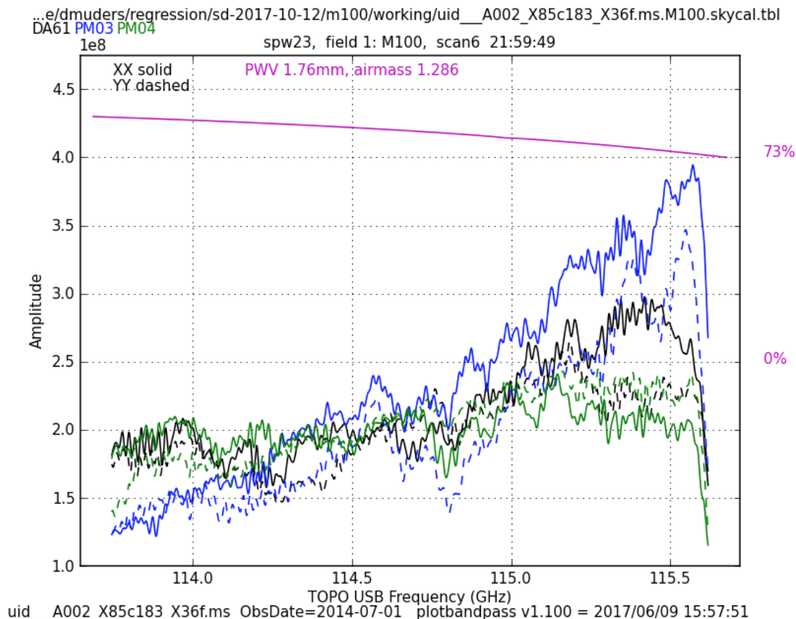
Figure 51: An example of an OFF spectrum. Different antennas are shown in different colors. The atmospheric transmission curve is shown in magenta.
