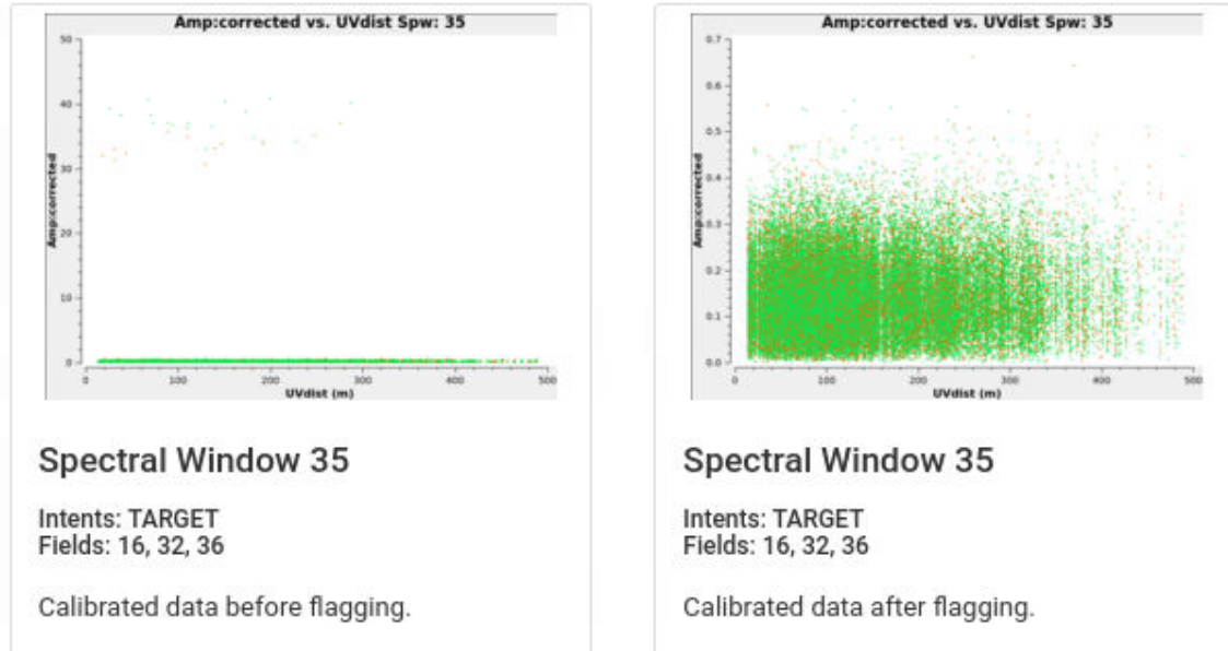
Figure 33: Example flagging of high outliers in science target visibilities in hifa_targetflag .
