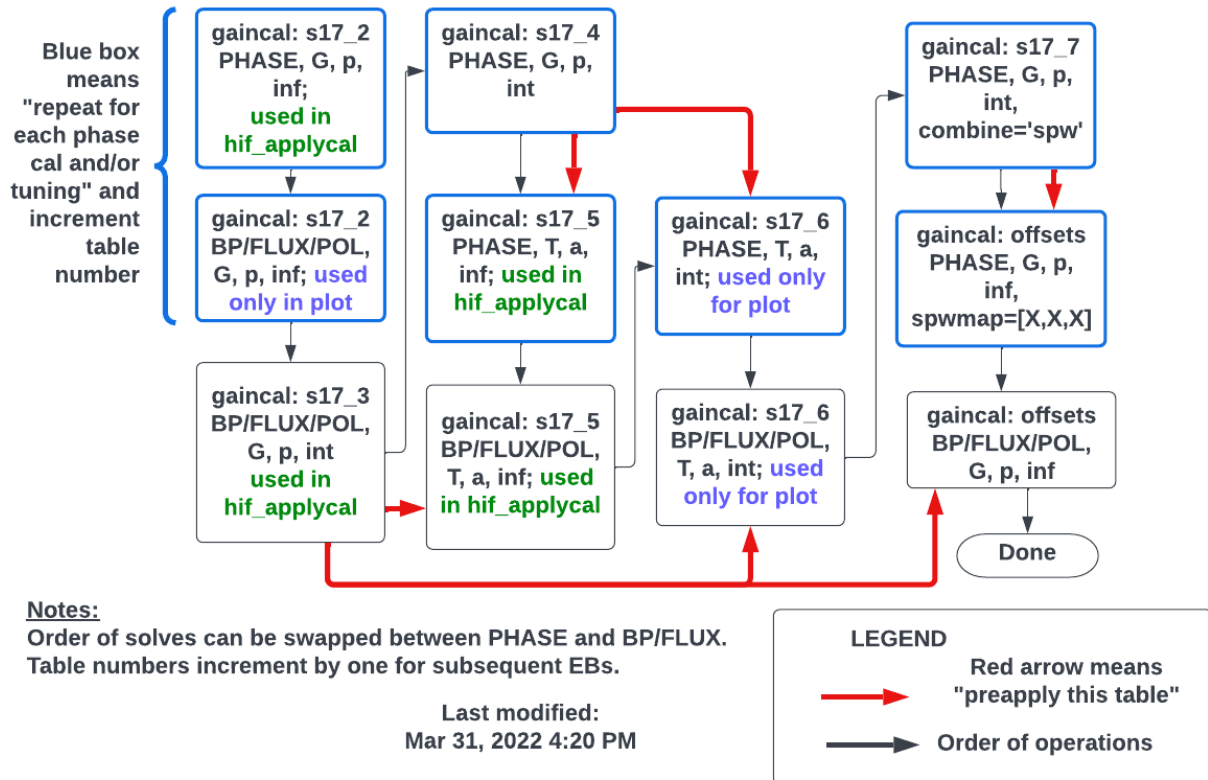
Figure 30: Logical flow in hifa_timegaincal for the case of high SNR in all spws.
