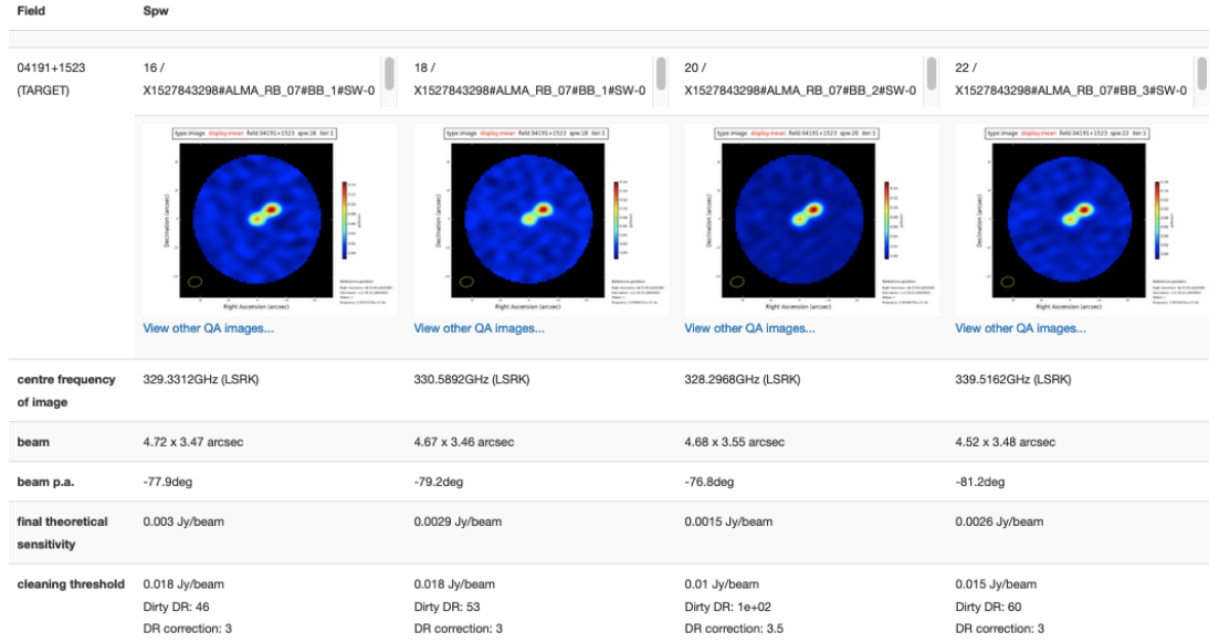
Figure 44: Example of hif_makeimages stage for per-spw continuum images. Clicking on the thumbnail will enlarge the image. Clicking the View other QA images link will bring up the detailed image page (Figure 45).
