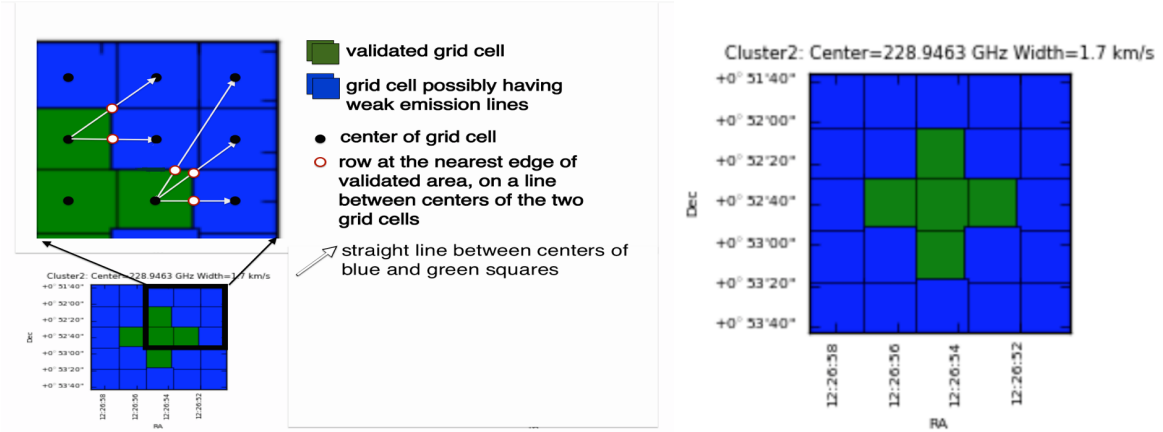
Figure 56: (a) An example of how the mask range is calculated. In the blue squares, the mask channel range is the range obtained at the nearest edge of any validated area by interpolating mask channel ranges in the valid grid cells (white-filled red circle). (b) An example of clustering_final.
