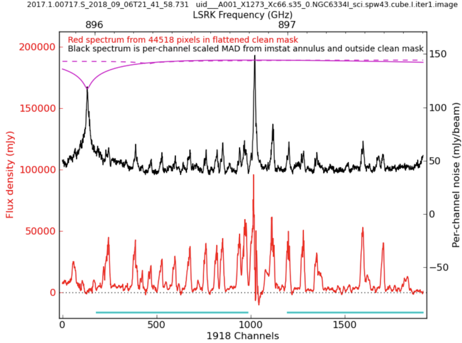
Figure 48: Example of a cube spectrum (red) constructed from pixels inside the clean mask, overlaid with a noise spectrum (black) constructed from the (portion of the) noise annulus outside the clean mask.
