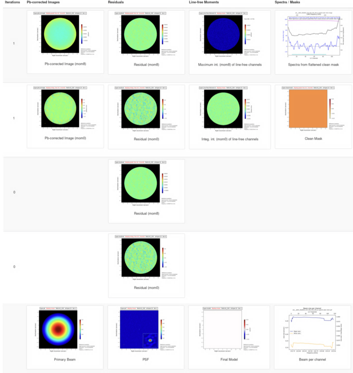
Figure 47: Example of an image cube details page including the line-free moment 0 and moment 8 images.
