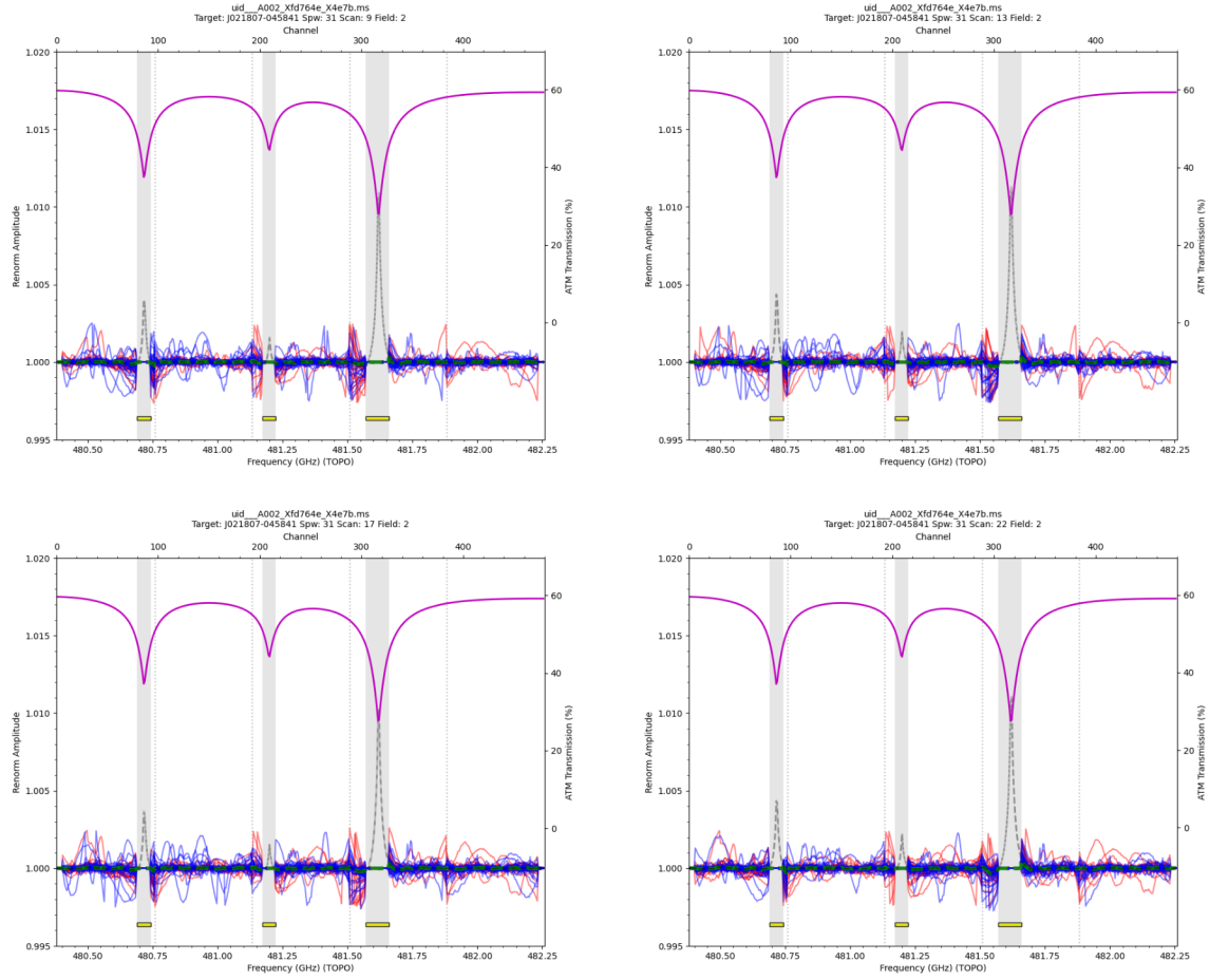
Figure 42: Screenshot of a PDF file as Figure 41 but where atmospheric regions have been automatically excluded and are covered by semi-opaque grey regions. It is clear to see that the excluded scaling spectra (visible by the grey dashed lines) are coincident with the three deep atmospheric lines shown by the magenta line. The section of frequencies (channels) that will be excluded are also illustrated by the yellow boxes towards the bottom of each plot. In this example renormalization will not be applied as there are no real astronomical lines to scale.
