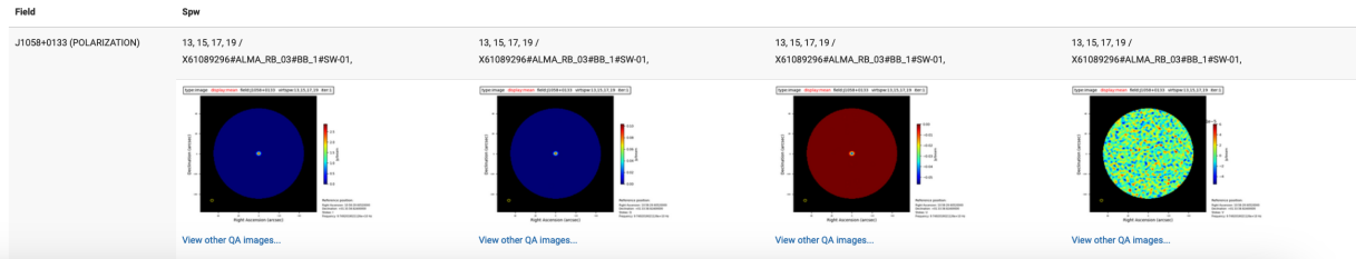
Figure 36: Example of the hif_makeimages stage for the Polarization calibrator (§9.27). First it displays the polarization fit results for each session along with the polarization intensity and angle plots, followed by Stokes I, Q, U, and V images. Clicking on the thumbnails will enlarge the image. Clicking the View other QA images link will bring up the detailed image page.
