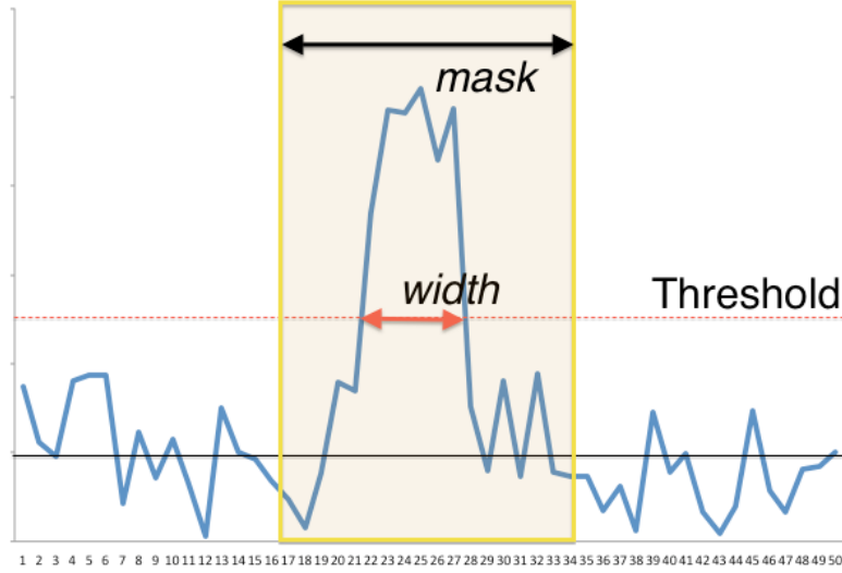
Figure 53: An example spectrum to explain Pipeline-defined mask range. “Width” corresponds to the number of channels where the emission is above the threshold.
