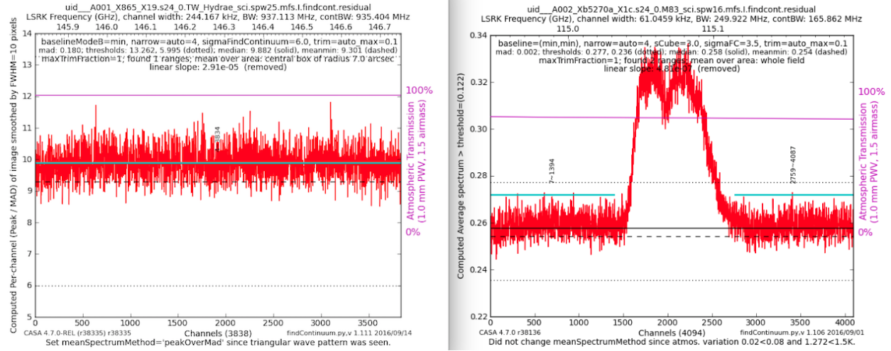
Figure 43: Two examples of hif_findcont plots, one with the entire window identified as continuum (left panel), and another with two identified continuum regions (right panel). The identified continuum range(s) are indicated by the horizontal cyan lines.
